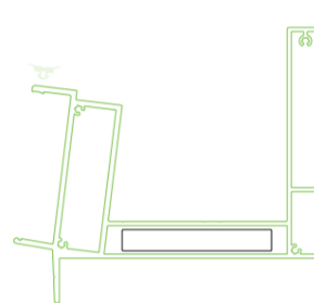
V001015 Blenda
